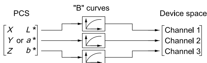
b) Using a lutBToAType model
