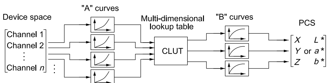
d) Using a lutAToBType model
