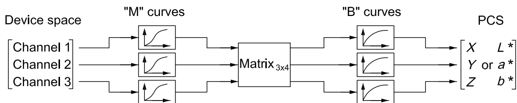
c) Using a lutAToBType model
